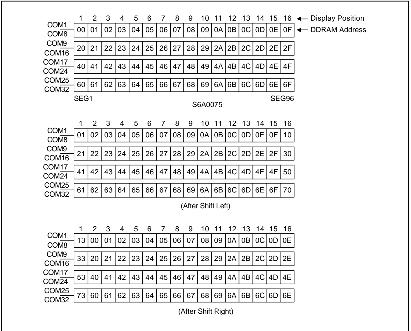
Figure 7. 4-line 16ch. Display (6-dot Font Width)
