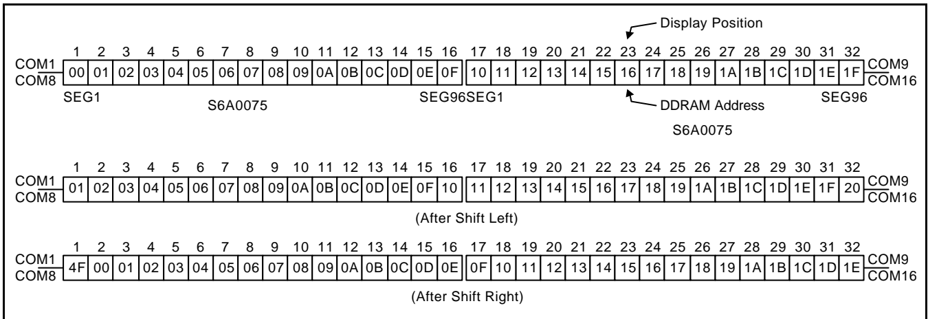
Figure 5. 1-line 32ch. Display
