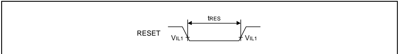
Figure 18. Reset Timing Diagram
