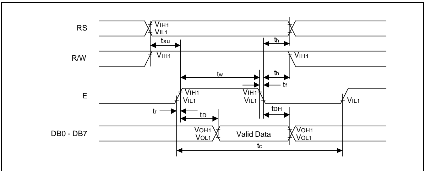
Figure 16. Read Mode
