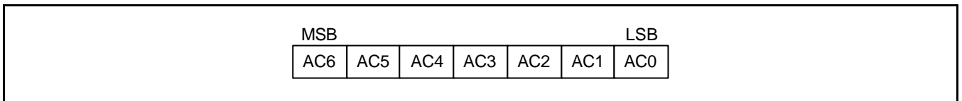
Figure 1. DDRAM Address
