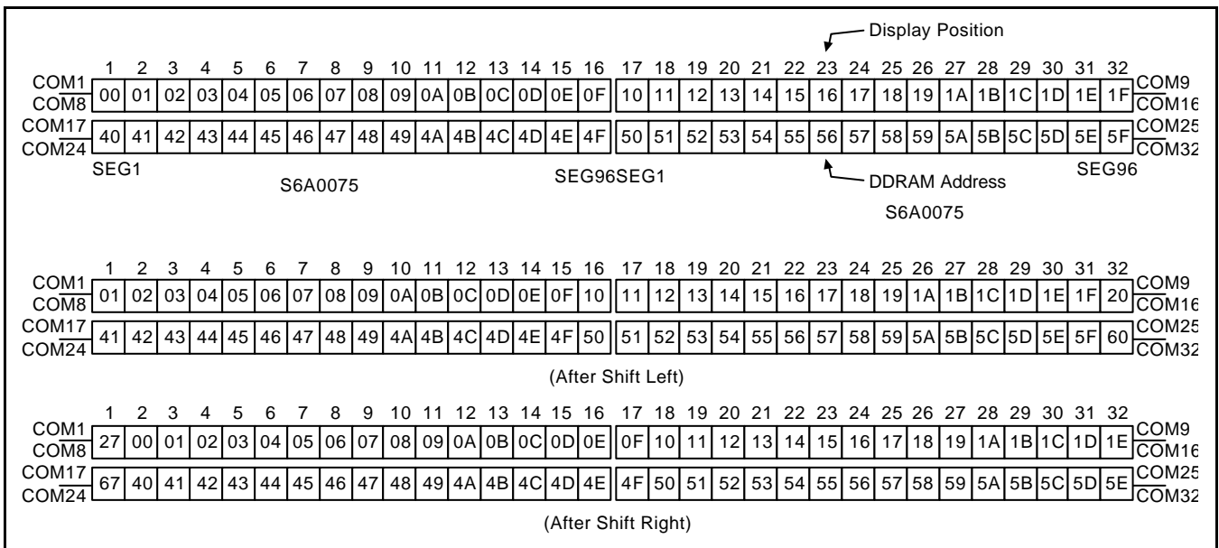
Figure 6. 2-line 32ch. Display (6-dot font width)
