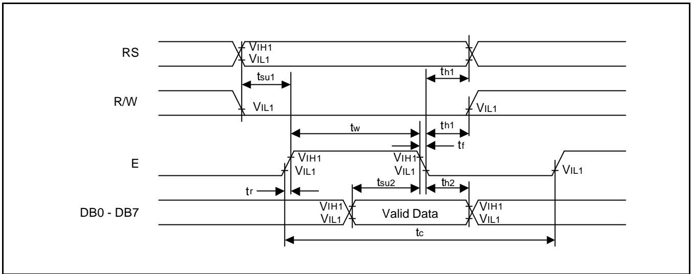
Figure 15. Write Mode
