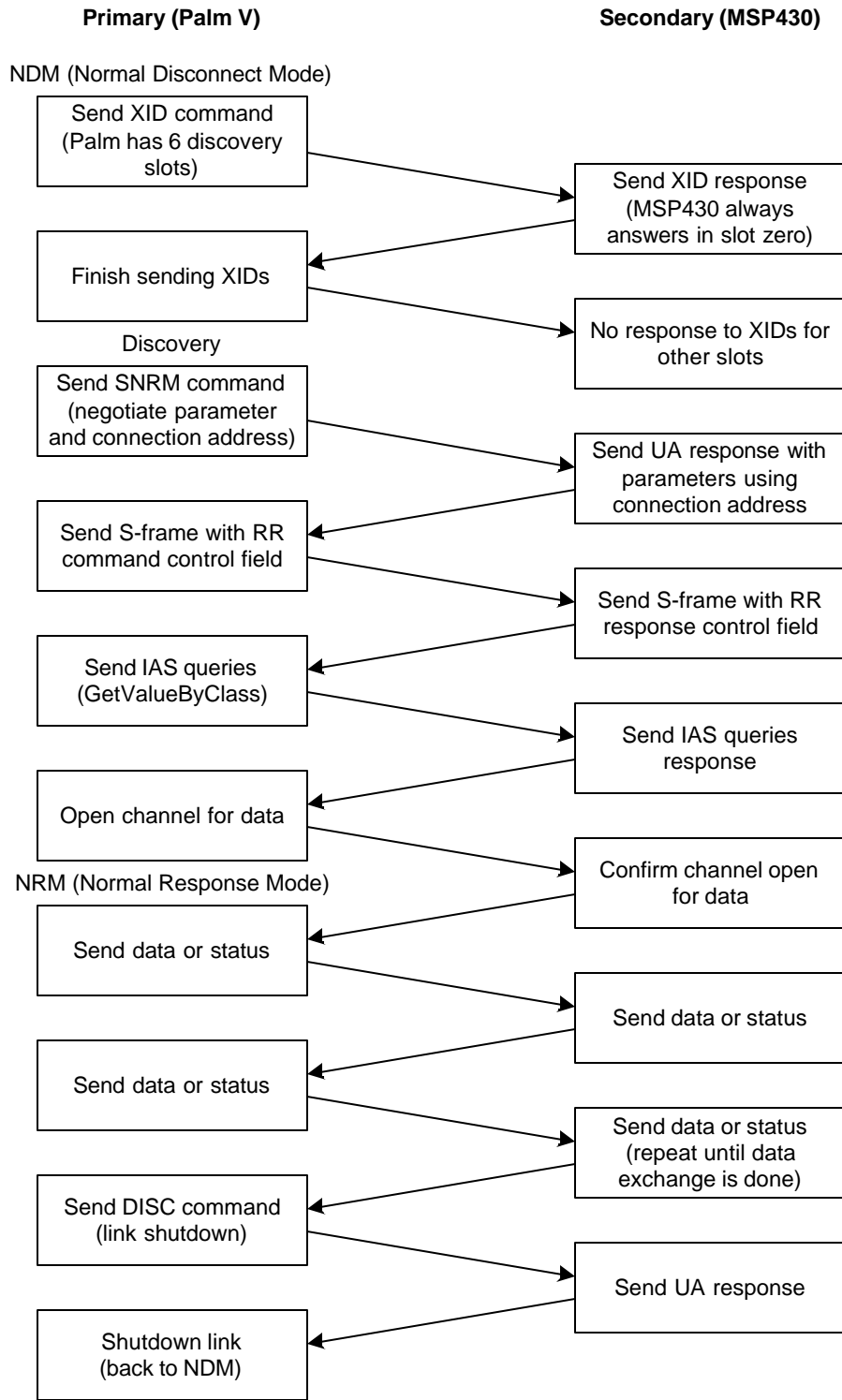
Figure 19. IrDA Communication Diagram
