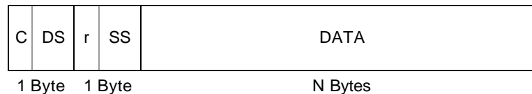
Figure 17. IrLMP Frame Format
