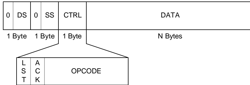
Figure 12. IAP Frame Format
