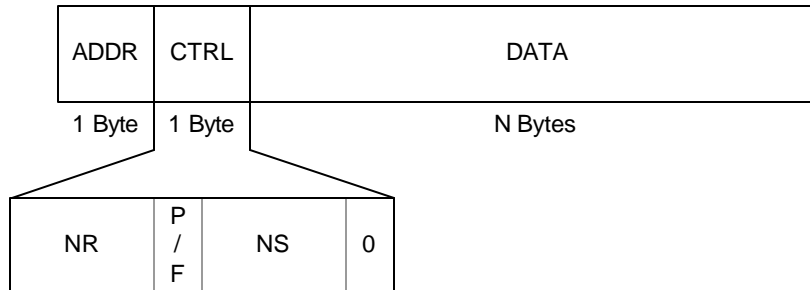
Figure 8. Information Frame Format
