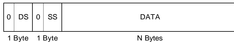
Figure 11. IrLMP Data Transfer Frame Format
