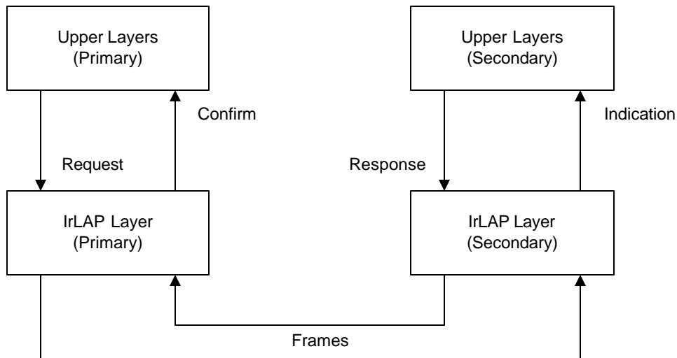
Figure 16. IrLAP Service Primitives
