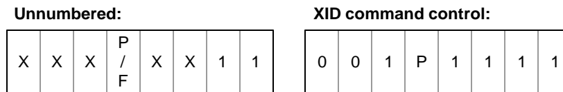
Figure 5. Unnumbered and XID Command Frame Formats
