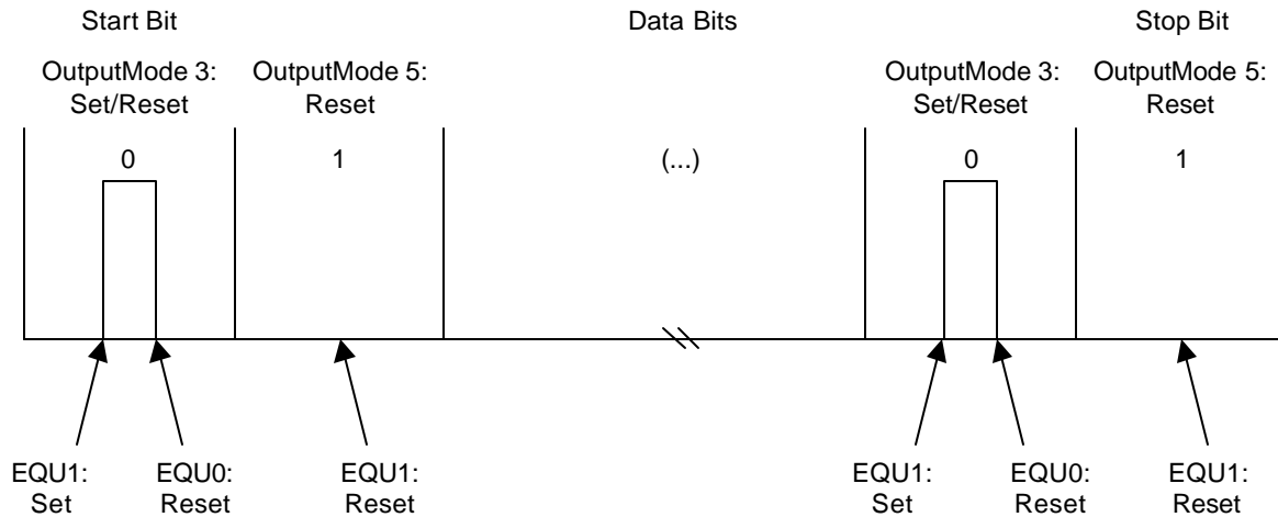
Figure 3. Transmission With Timer_A
