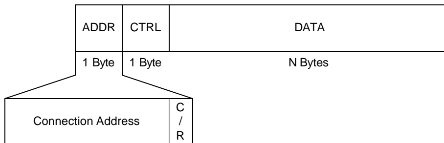
Figure 15. IrLAP Frame Format
