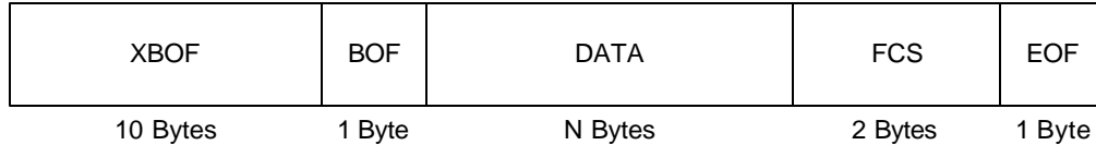
Figure 14. IrPHY Frame
