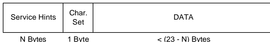
Figure 10. Device Information Field Format
