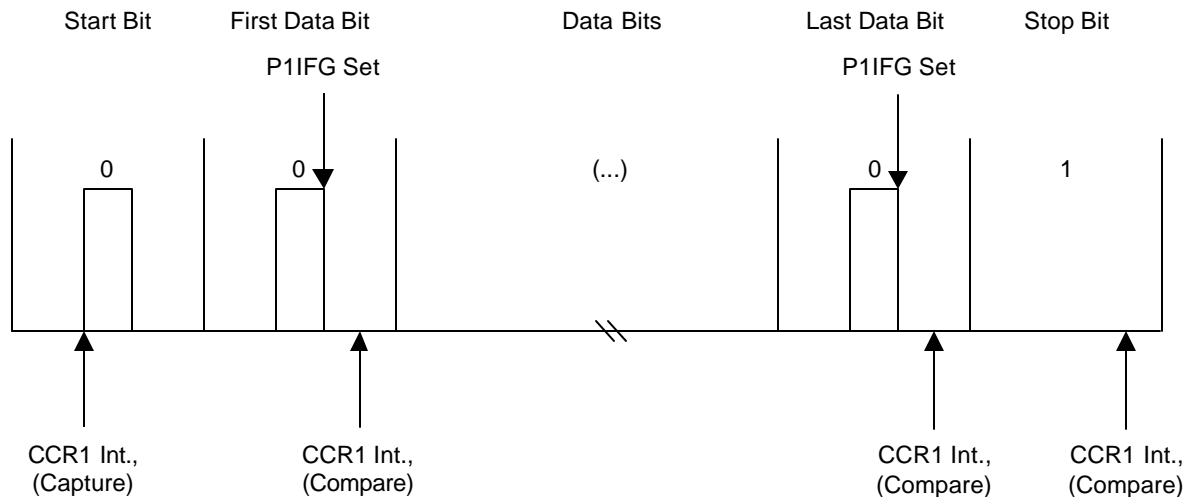
Figure 4. Detailed Byte Reception
