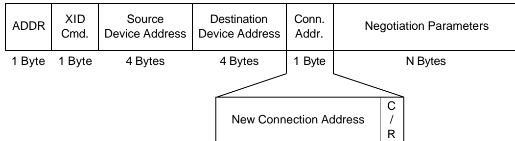
Figure 7. SNRM Frame Format
