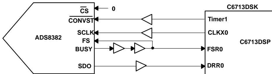
Figure 1. Hardware Connection
