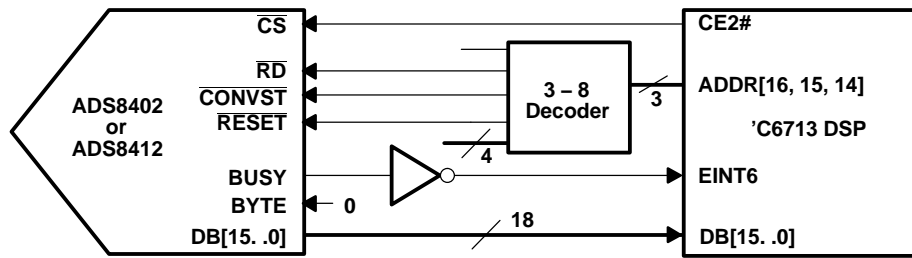
Figure 1. Hardware Connection
