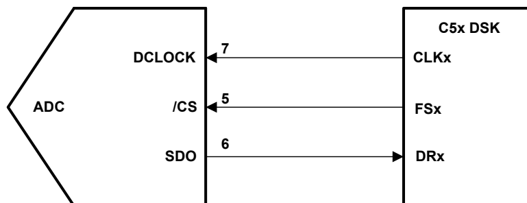
Figure 1. Hardware Interface Block Diagram
