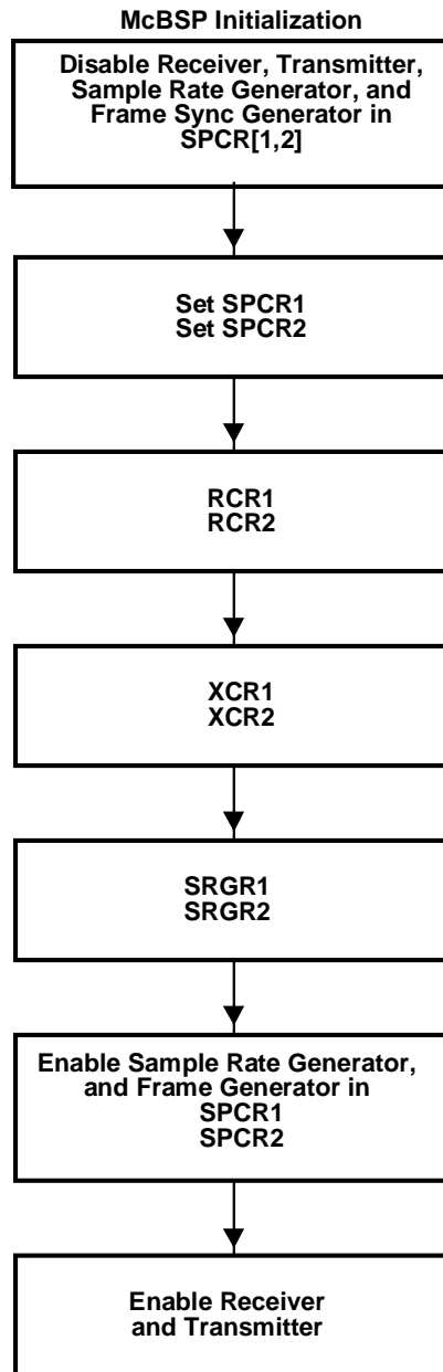
Figure 2. McBSP Programming
