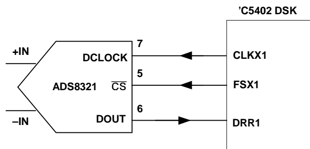
Figure 1. Hardware Interface Block Diagram
