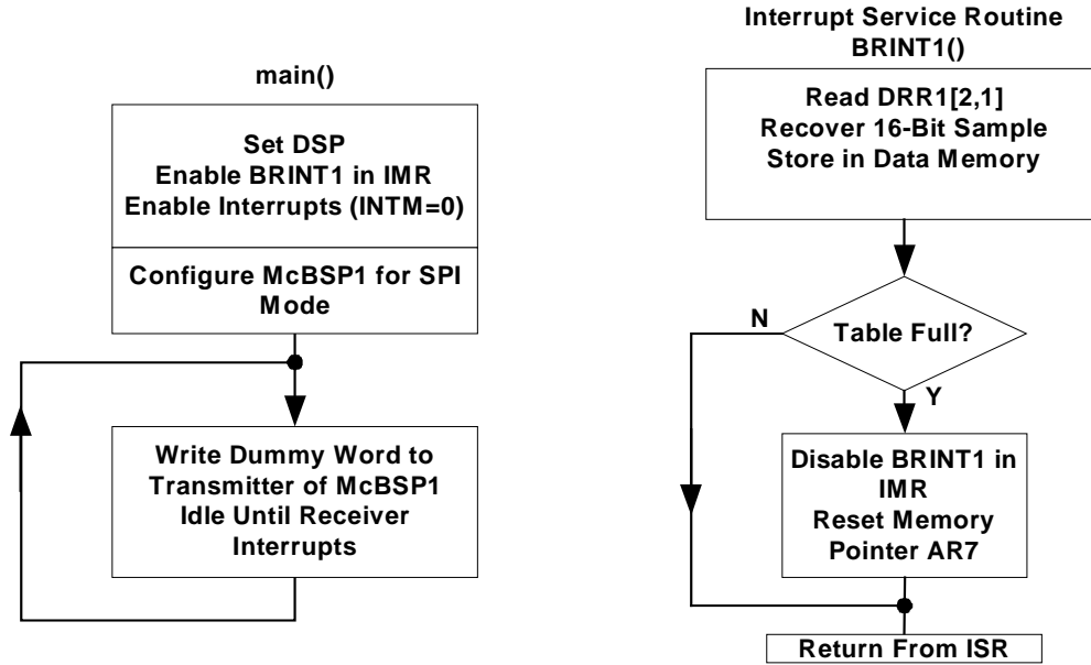
Figure 4. Software Flowchart
