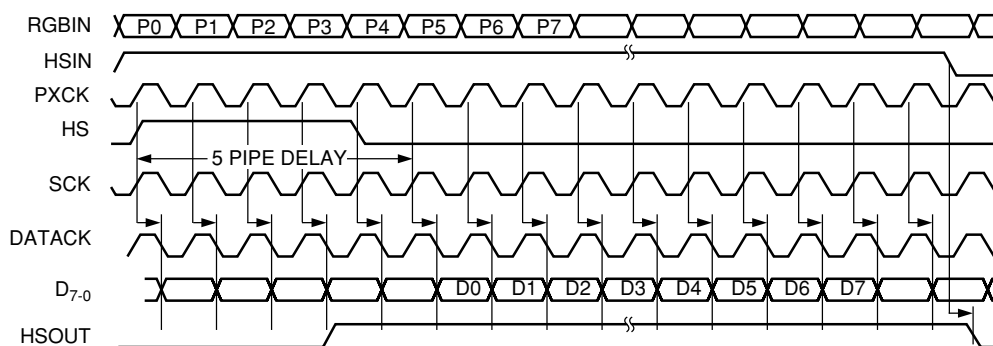
Figure 8. Normal Mode
