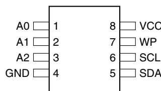
8-lead SOIC
