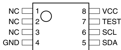
8-lead TSSOP
