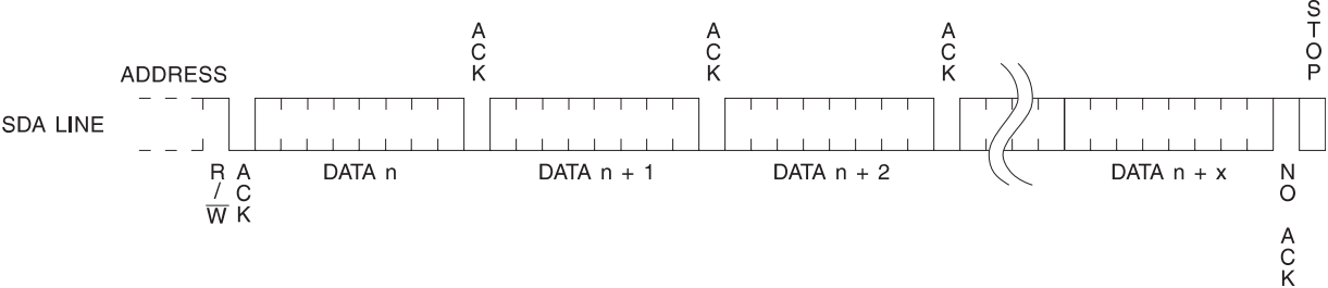
Figure 10. Sequential Read
