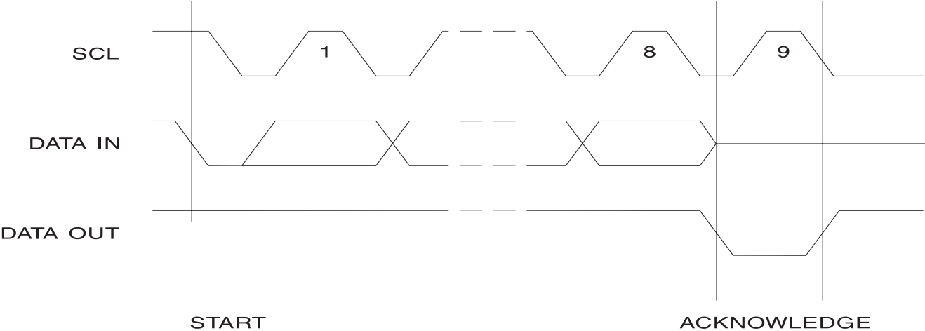
Figure 6. Output Acknowledge
