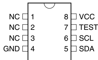
8-lead PDIP
