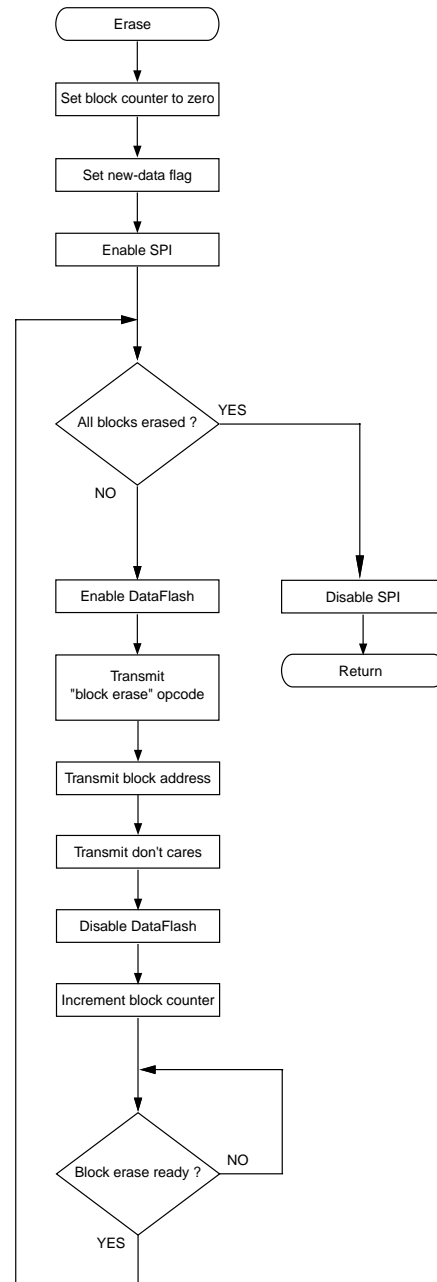
Figure 12. Erase
