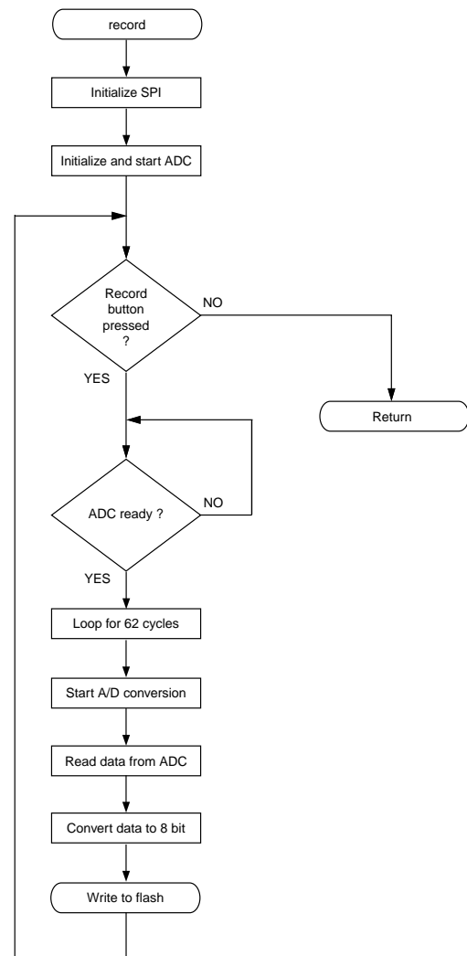
Figure 13. Record
