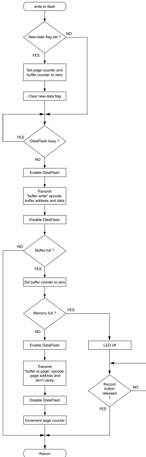
Figure 14. Write to DataFlash
