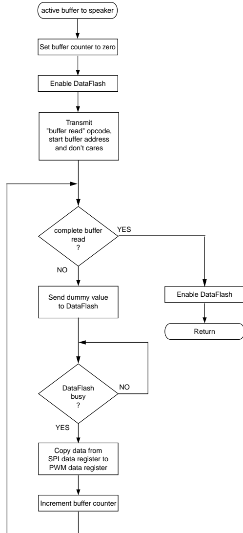
Figure 17. Active Buffer to Speaker
