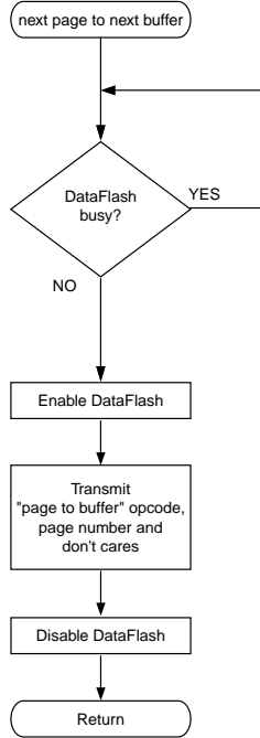
Figure 16. Next Page to Next Buffer
