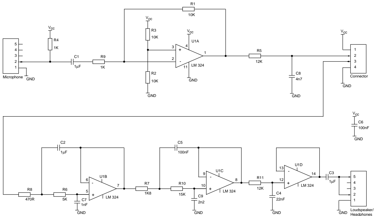
Figure 10. Microphone and Speaker Circuit Diagram
