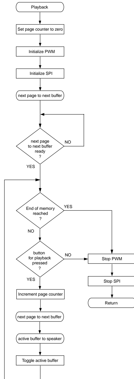
Figure 15. Playback
