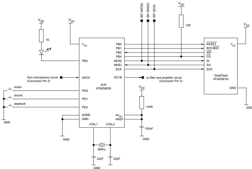
Figure 9. Microcontroller and Memory Circuit Diagram
