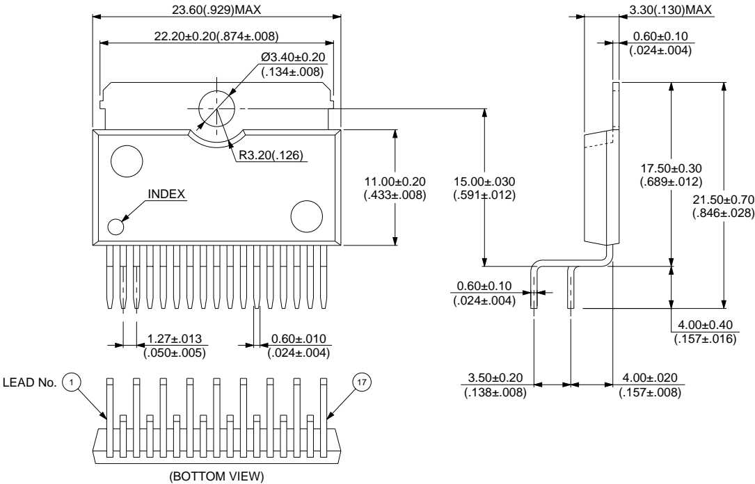
17-pin plastic ZIP (ZIP-17P-M03)
