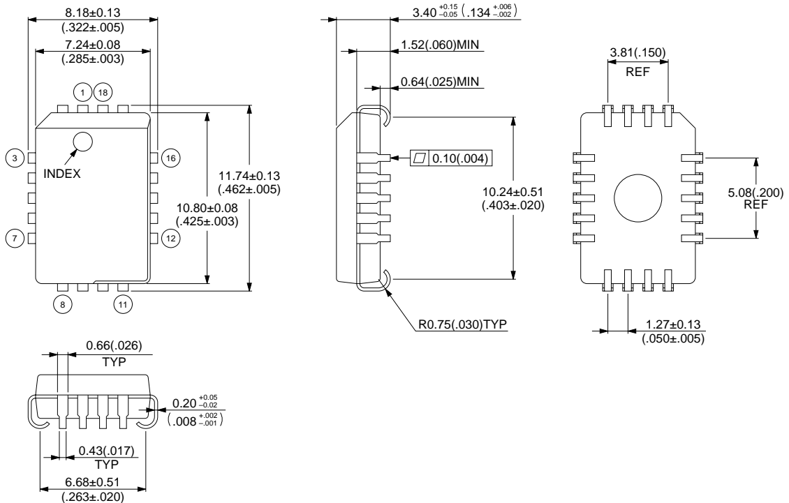
18-pin plastic QFJ (PLCC) (LCC-18P-M03)
