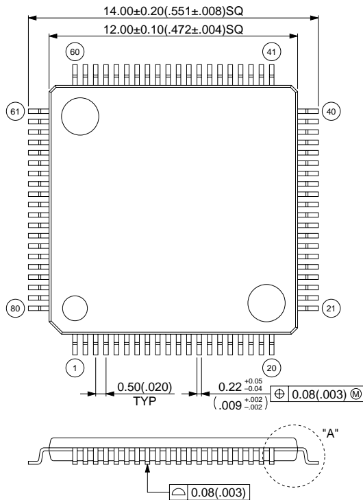
80-pin plastic TQFP (FPT-80P-M15)
