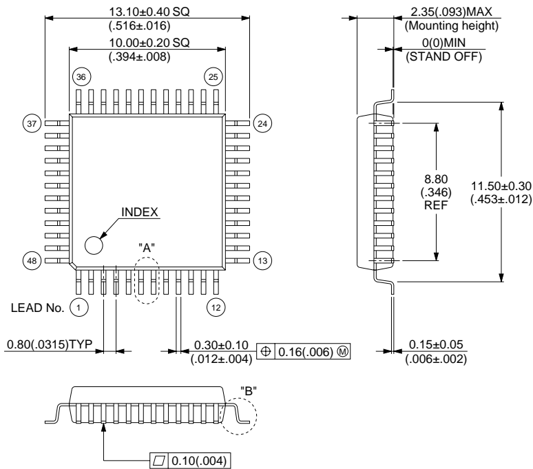
48-pin plastic QFP (FPT-48P-M13)
