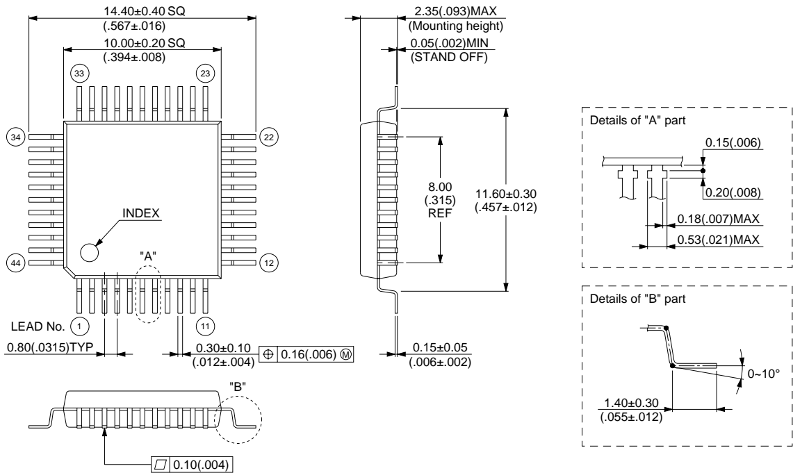
44-pin plastic QFP (FPT-44P-M11)
