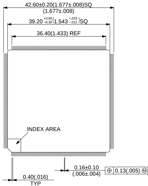
368-pin ceramic QFP (FPT-368C-C01)
