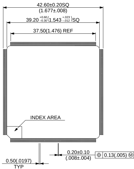
304-pin ceramic QFP (FPT-304C-C02)
