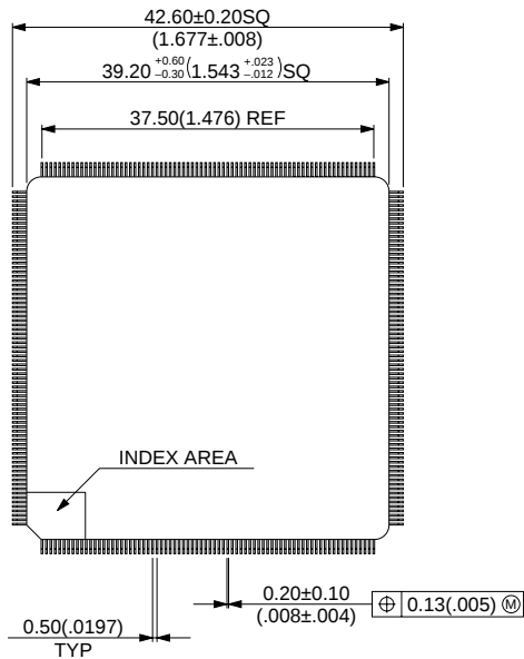
304-pin ceramic QFP (FPT-304C-C01)
