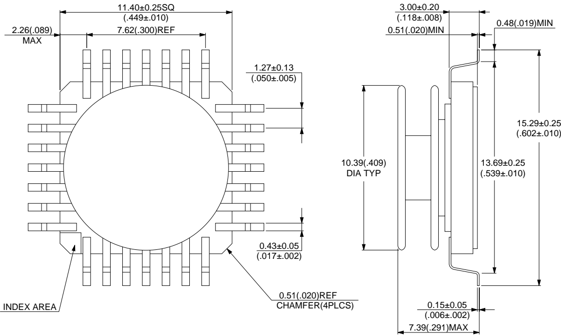
28-pin ceramic QFP (FPT-28C-A07)
