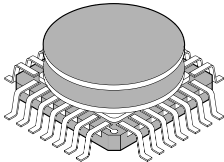
28-pin ceramic QFP
