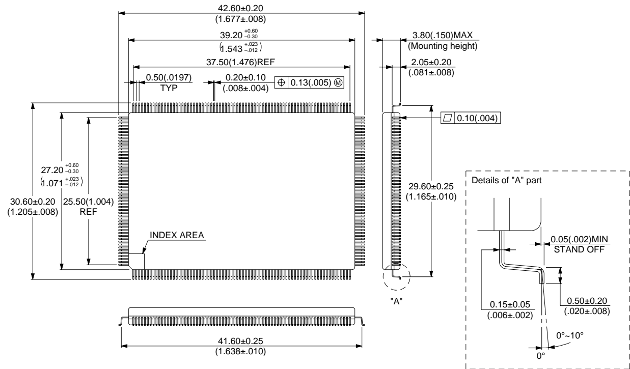
256-pin ceramic QFP (FPT-256C-C02)
