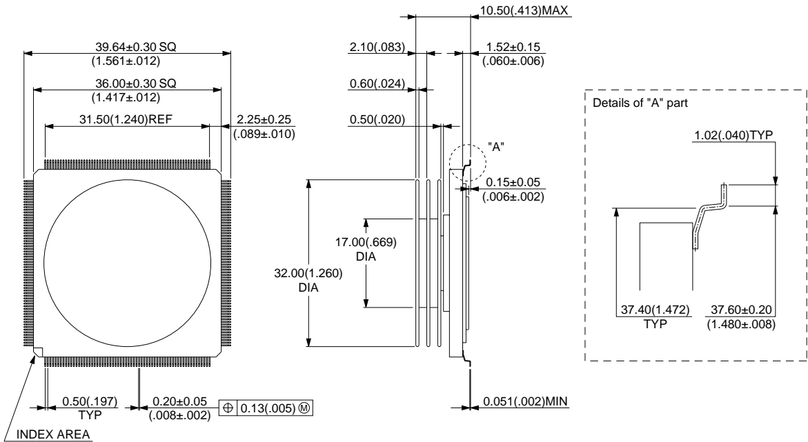
256-pin ceramic QFP (FPT-256C-A07)
