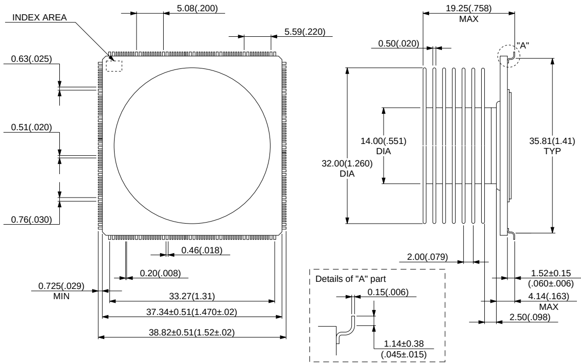
240-pin ceramic QFP (FPT-240C-A05)
