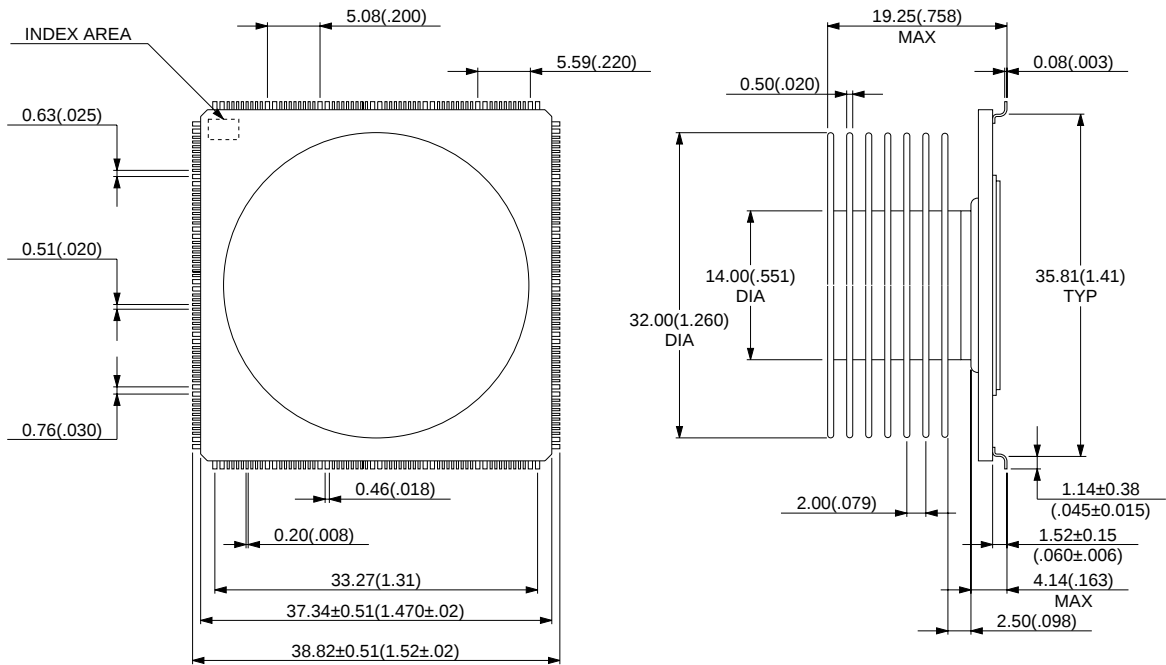
240-pin ceramic QFP (FPT-240C-A03)
