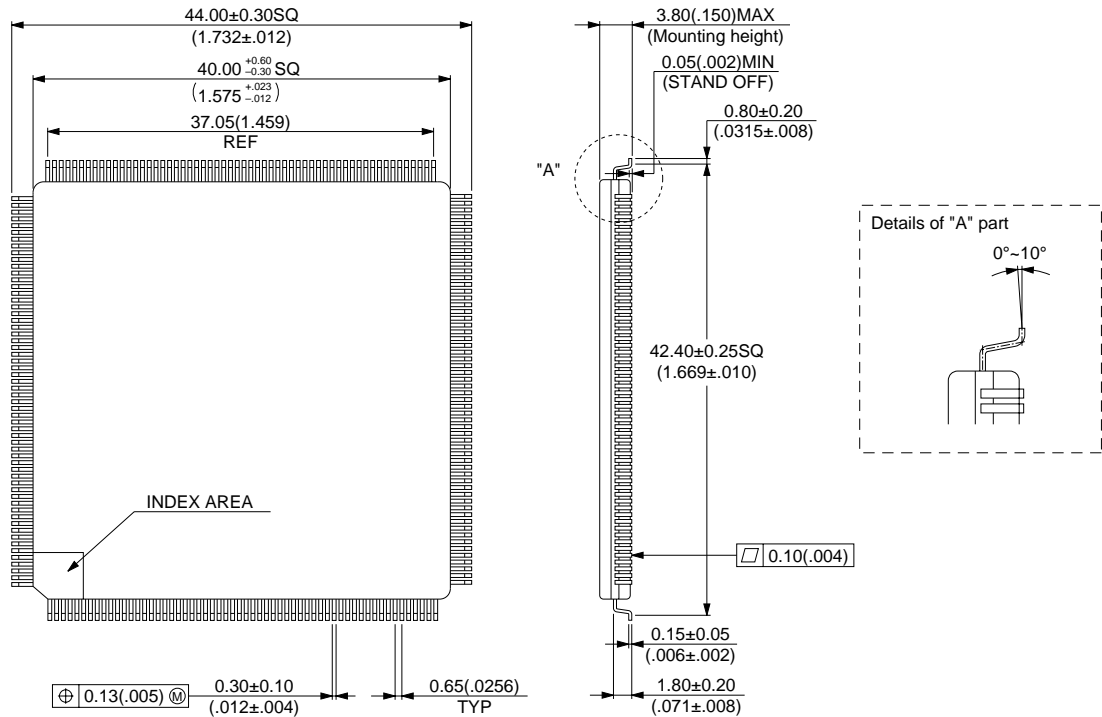
232-pin ceramic QFP (FPT-232C-C01)
