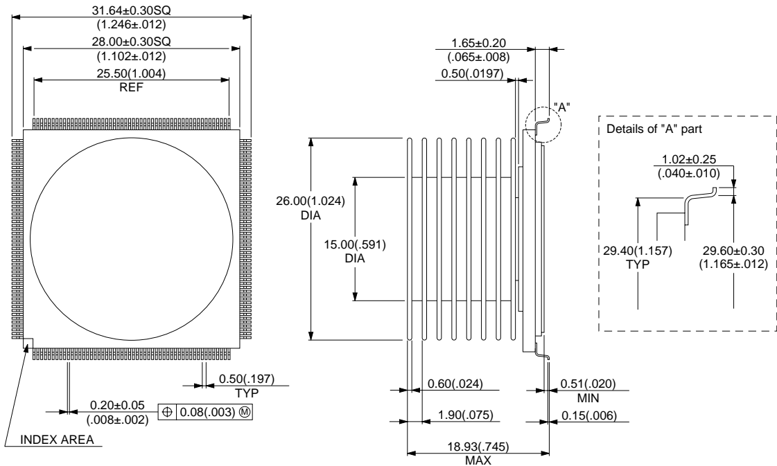
208-pin ceramic QFP (FPT-208C-A01)
