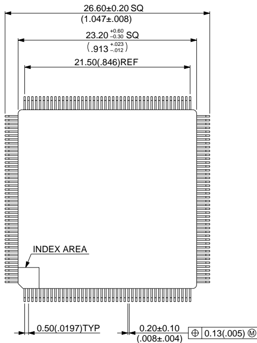
176-pin ceramic QFP (FPT-176C-C01)
