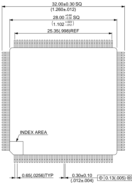
160-pin ceramic QFP (FPT-160C-C04)
