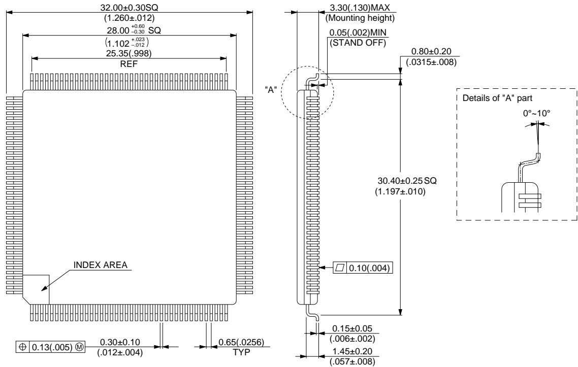
160-pin ceramic QFP (FPT-160C-C01)
