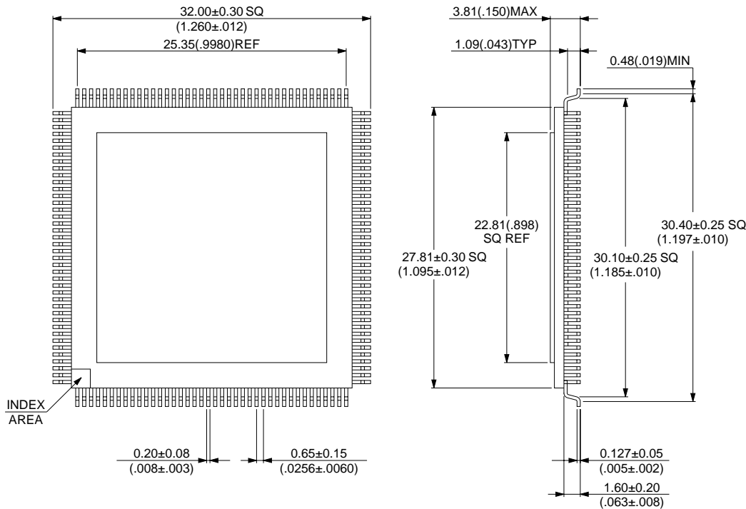
160-pin ceramic QFP (FPT-160C-A01)
