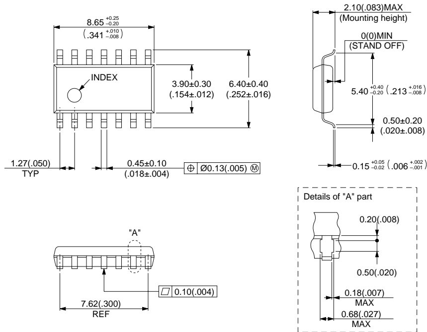
14-pin plastic SOP (FPT-14P-M03)
