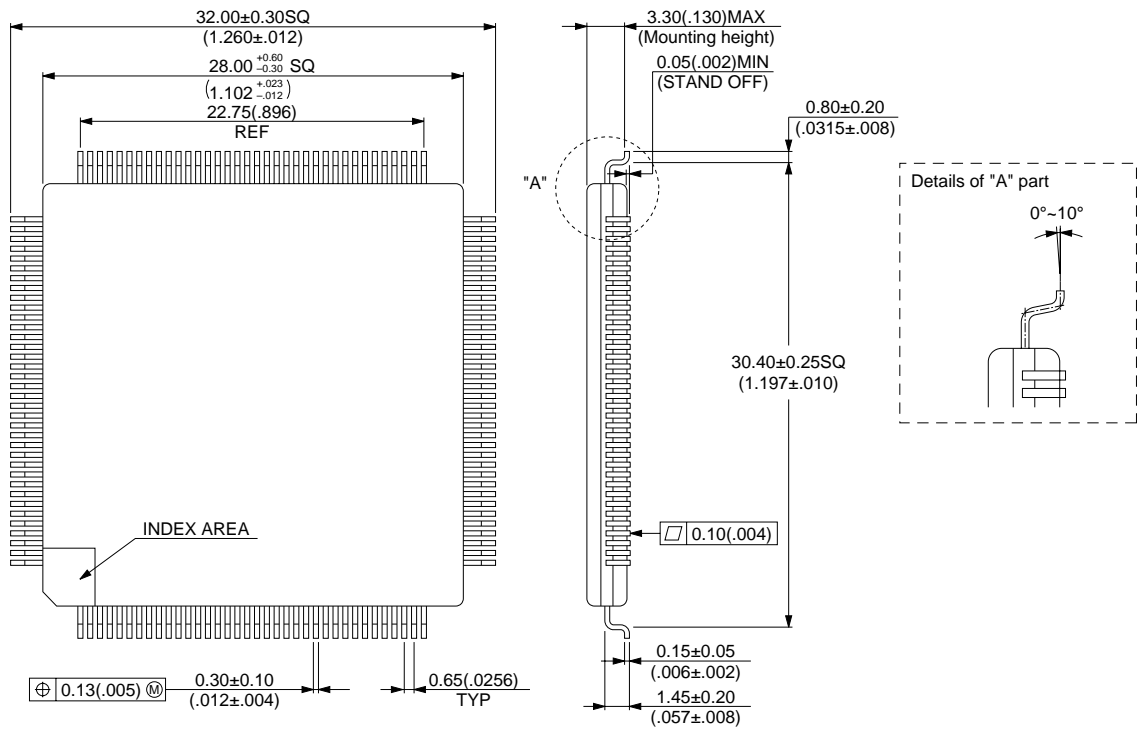
144-pin ceramic QFP (FPT-144C-C01)
