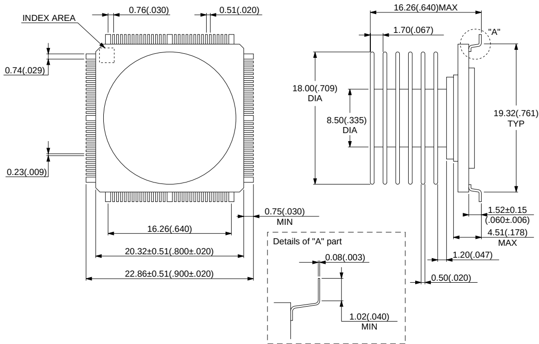
124-pin ceramic QFP (FPT-124C-A03)
