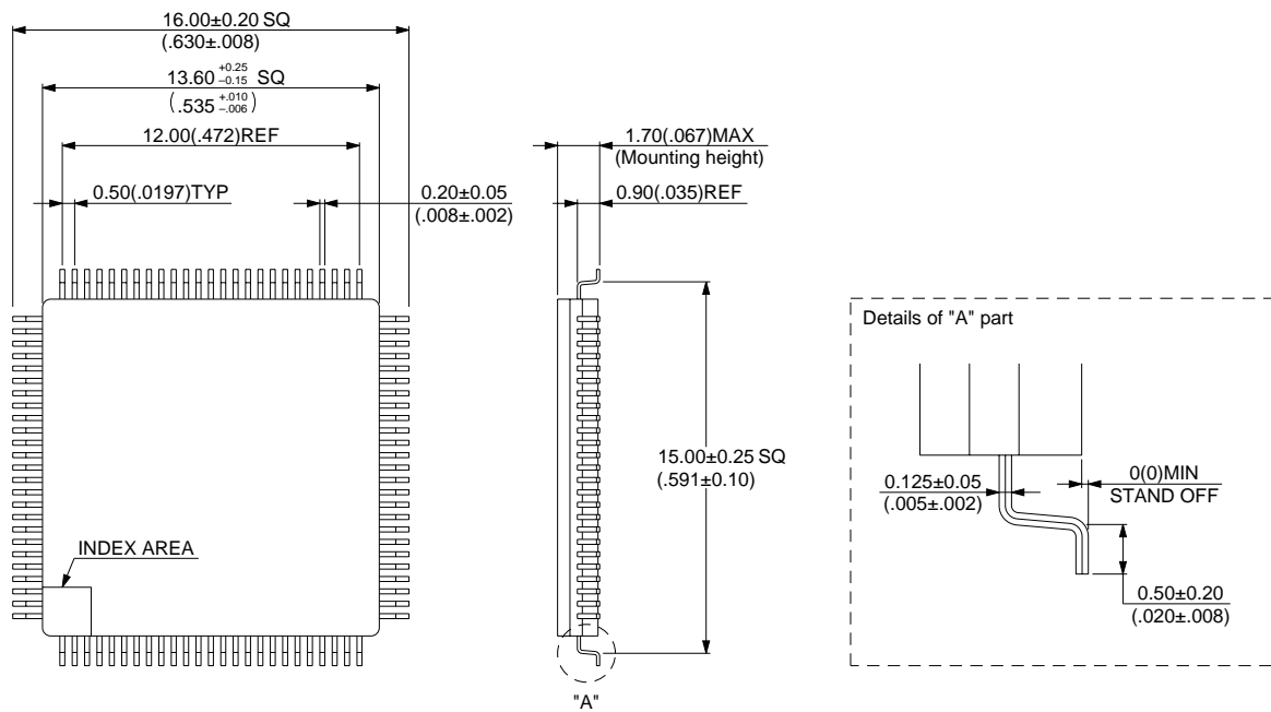
100-pin ceramic LQFP (FPT-100C-C01)
