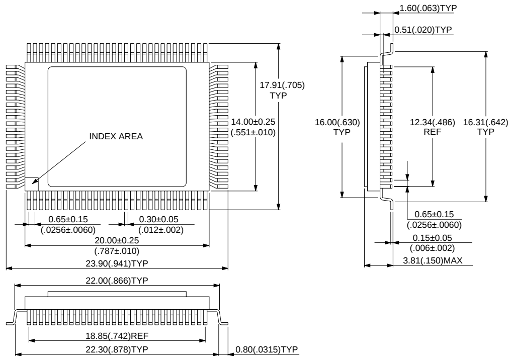
100-pin ceramic QFP (FPT-100C-A01)
