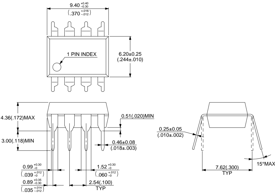
8-pin plastic DIP (DIP-8P-M01)
