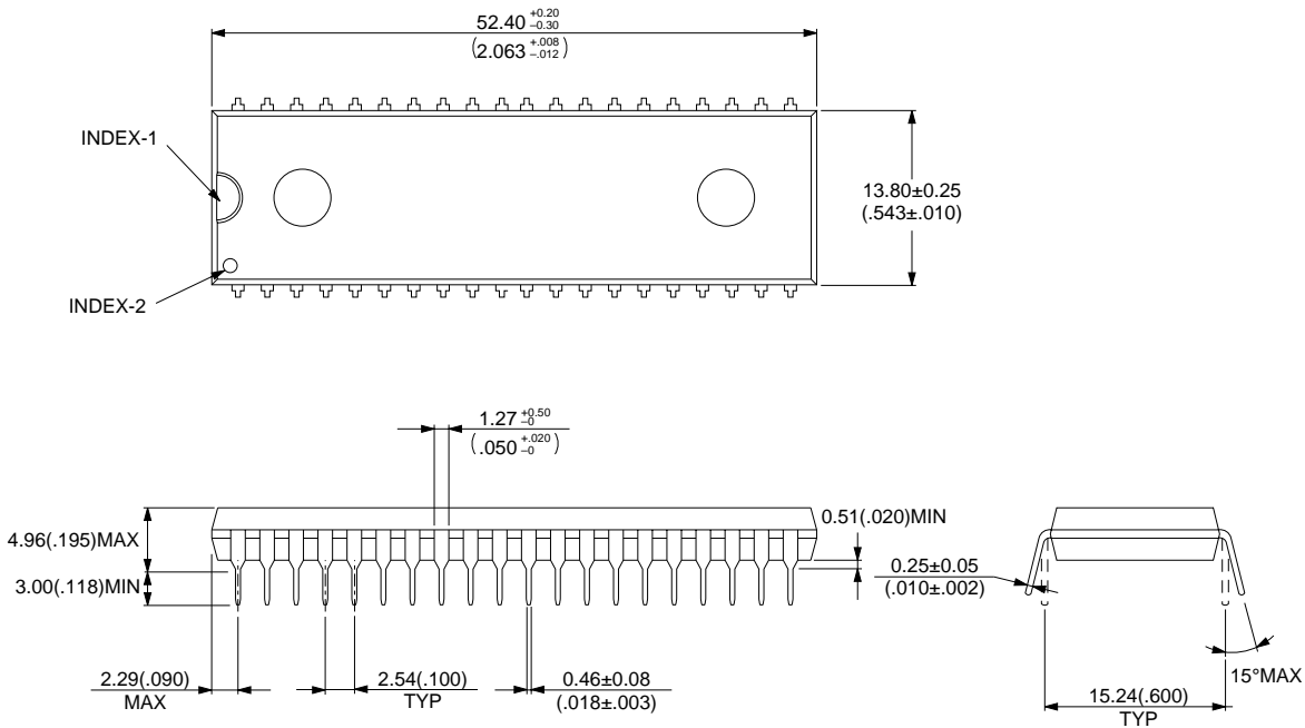
40-pin plastic DIP (DIP-40P-M02)
