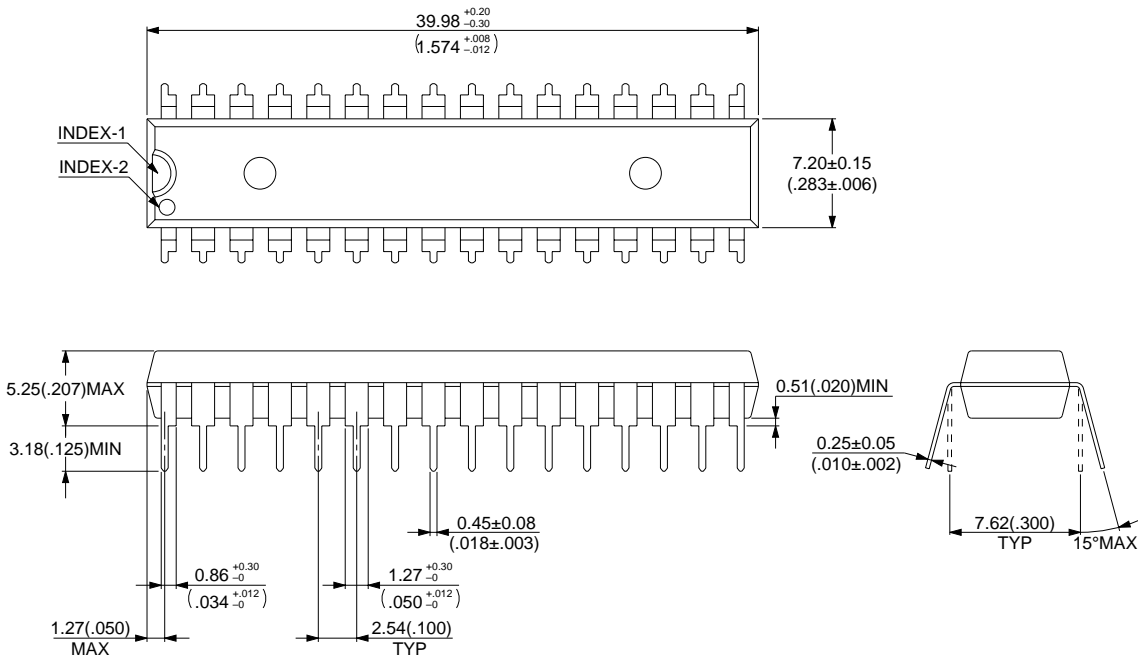
32-pin plastic SK-DIP (DIP-32P-M02)
