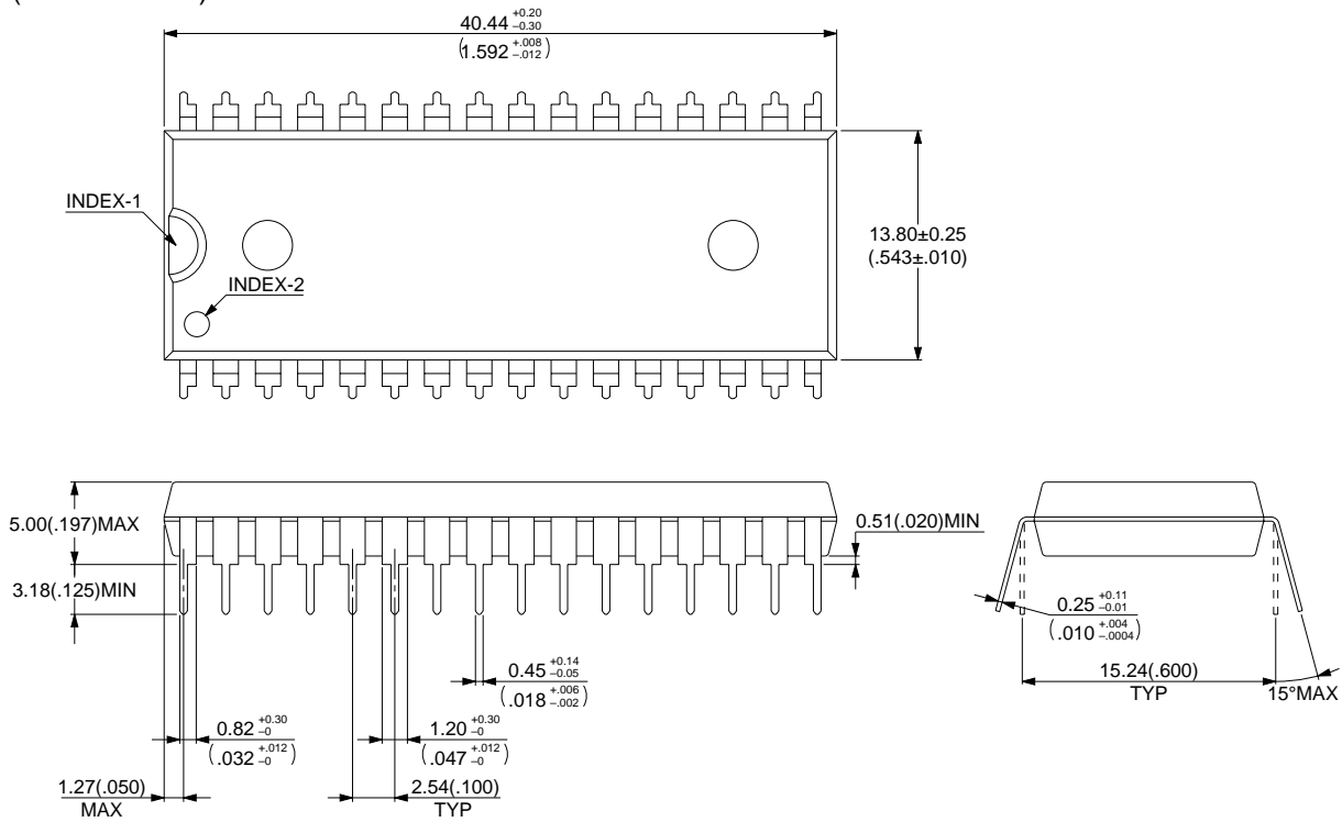
32-pin plastic DIP (DIP-32P-M01)
