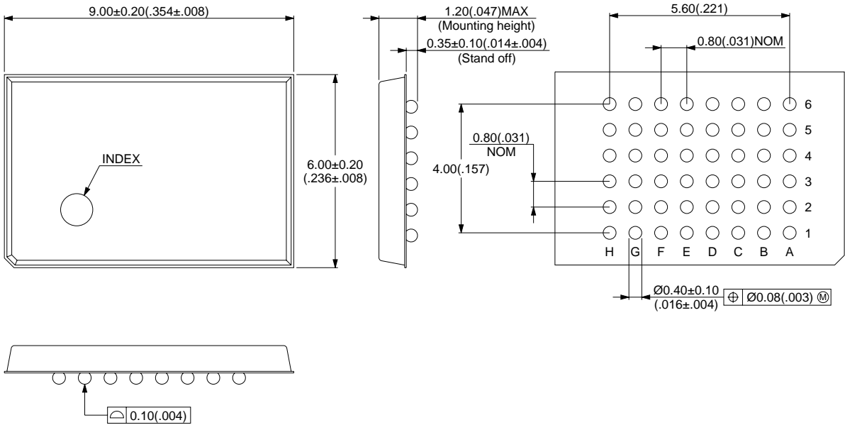
48-pin plastic FBGA (BGA-48P-M02)
